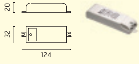
87 POWER SUPPLY 10W/110÷240V - 24Vdc IP20 CLASS II SELV.
