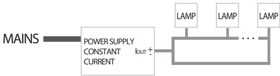
Wiring Diagram and sample series installation n.1
