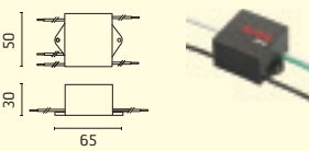
237 SPD: (SURGE PROTECTION DEVICE) 275Vac MAXIMUM DISCHARGE CURRENT 10KA (8/20µs) MAXIMUM OPERATING CURRENT 5A SUITABLE FOR SERIES CONNECTION - IP66
