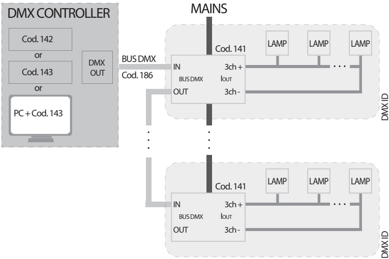
Wiring Diagram and sample installation n.5
