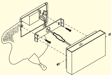
Optional: power supply code 106 in recessed box
