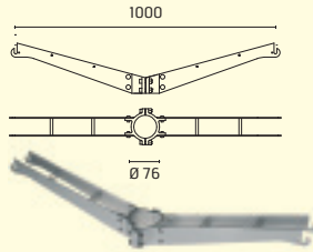
115 DOUBLE BRACKET 500mm FOR POLE Ø 76mm
