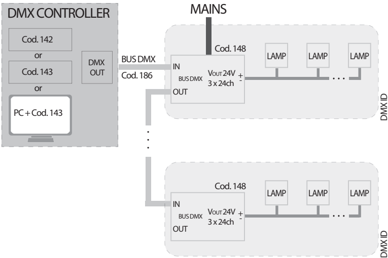
Wiring Diagram and sample installation n.6
