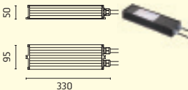
155 POWER SUPPLY 50W/120÷240V - 24Vdc IP67 CLASS II SELV.
