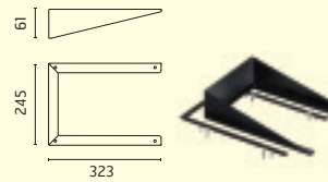
167 WALL WASHER VISOR
