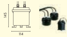
16 TRANSFORMER 50W 230V/12V 50Hz IP 66
